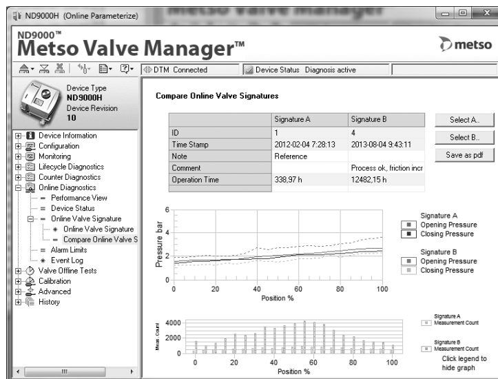
Figure 2. Valve Online Signature feature shows friction of the control valve online, under normal process conditions when ever the valve is changing position.
